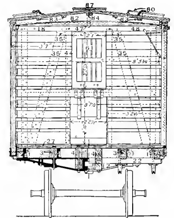
Fig. 372. Transverse Sections.
